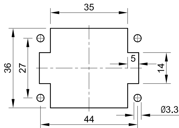
Panel cut out 面板开孔尺寸
